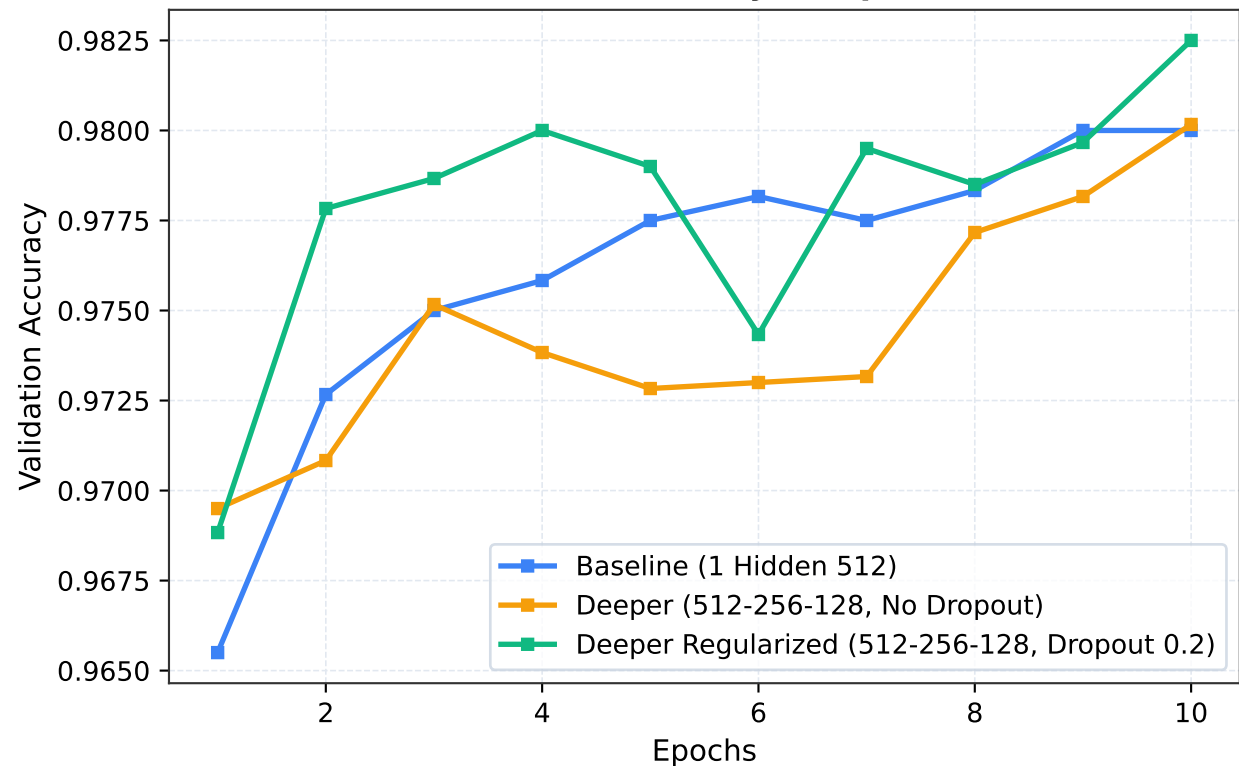
Validation Accuracy Comparison
