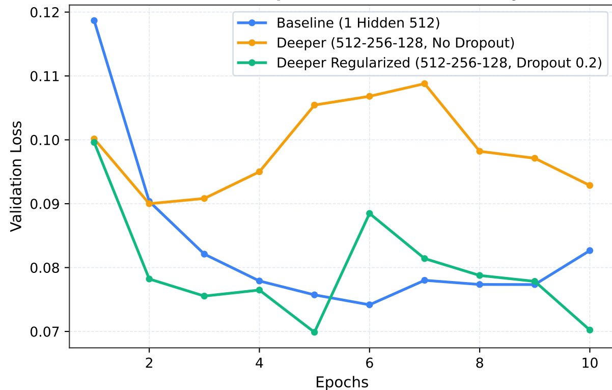
Validation Loss Comparison (Generalization Dynamics)
